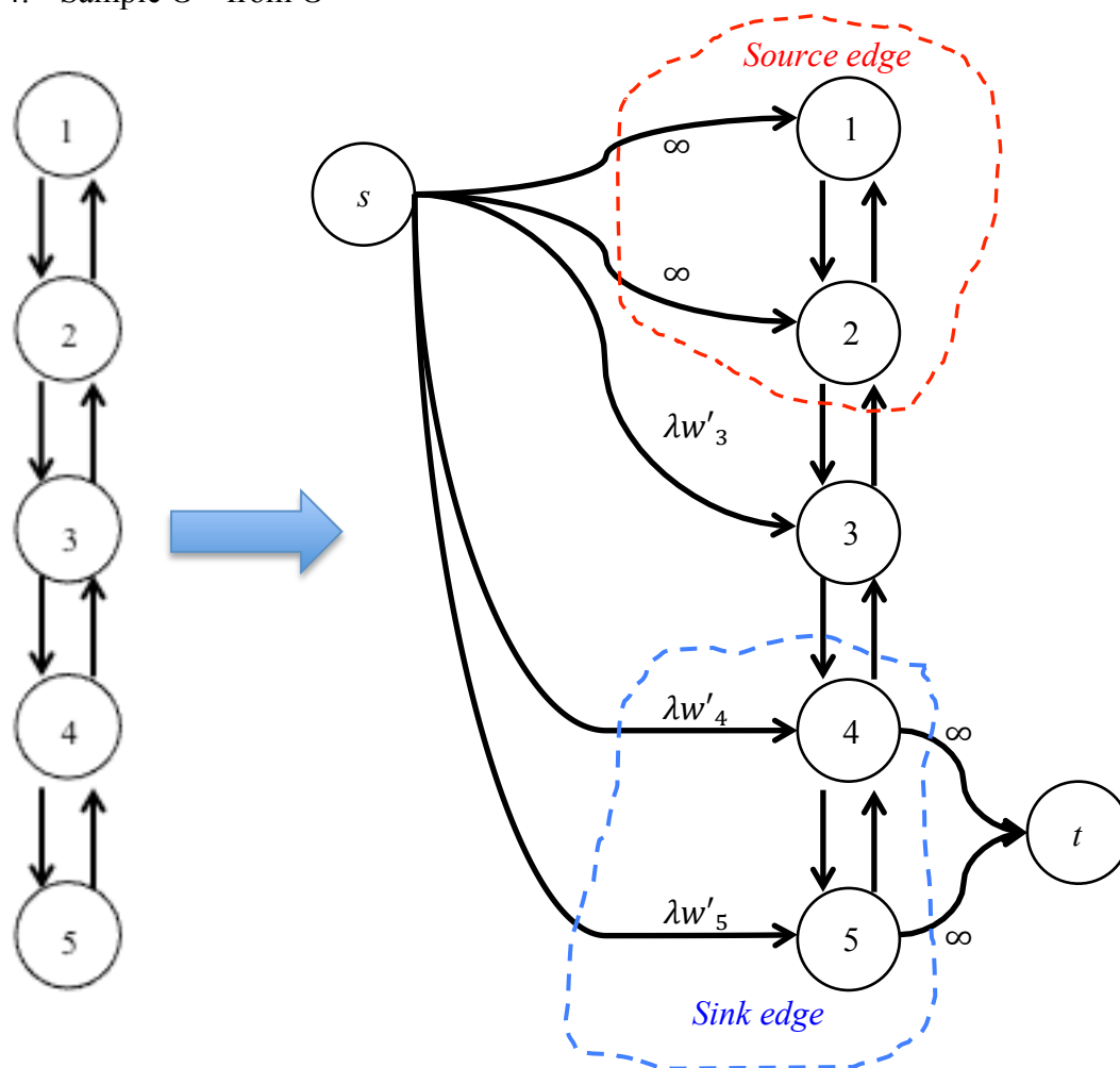
Figure 4: Sample G'' from G
